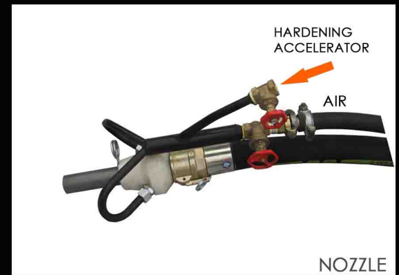
Wet method shotcreting
